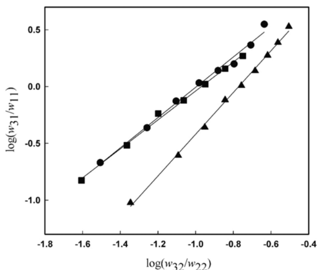
Fig. 5. Hand plots of o -xylene(1)+water(2)+butyric acid(3)+ethyl acetate(4) at 25 °C: \blacktriangle , o -xylene/ethyl acetate (75/25); \bullet , o -xylene/ethyl acetate (50/50); \blacksquare , o -xylene/ethyl acetate (25/75).
